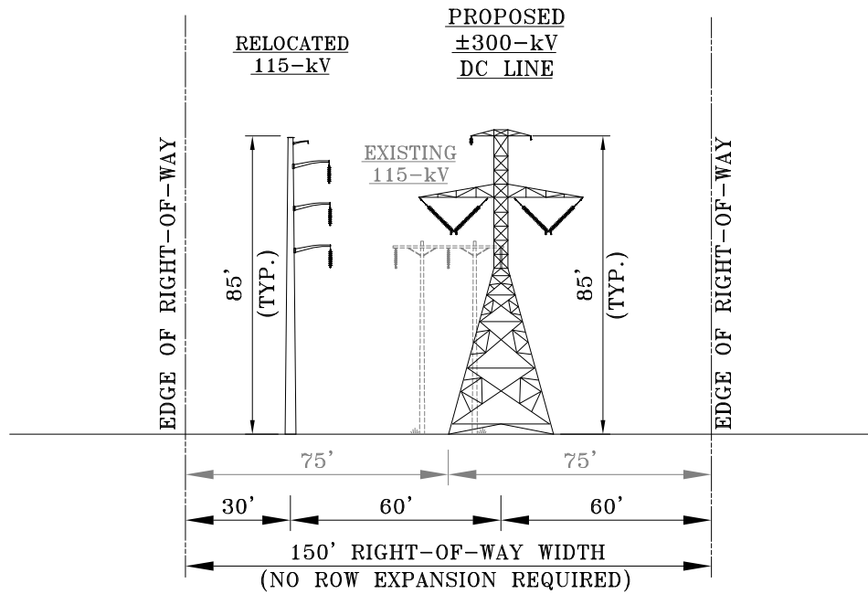
ROW CROSS SECTION WHITE MOUNTAIN NATIONAL FOREST
